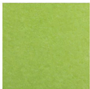
PEAR
